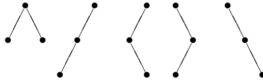
FIGURE 3. The five binary trees with 3 vertices.
