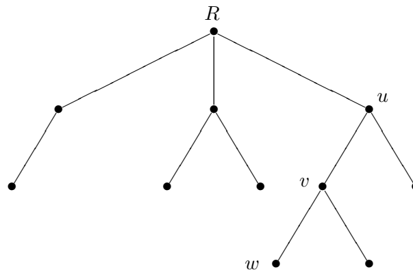
FIGURE 2. An example of a rooted tree.
