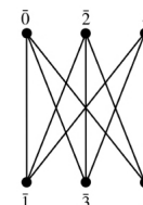
FIGURE 3. OD^3(\mathbb{Z}_6)
