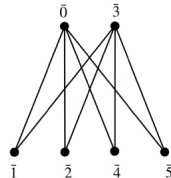
FIGURE 2. OD^2(\mathbb{Z}_6)
