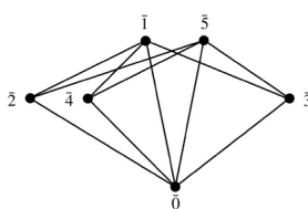
FIGURE 1. OD^1(\mathbb{Z}_6)
