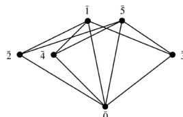
FIGURE 5. OD^5(\mathbb{Z}_6)
