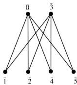
FIGURE 4. OD^4(\mathbb{Z}_6)
