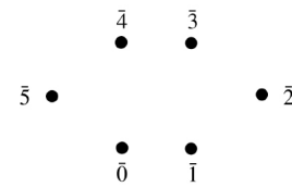
FIGURE 6. OD^6(\mathbb{Z}_6)
